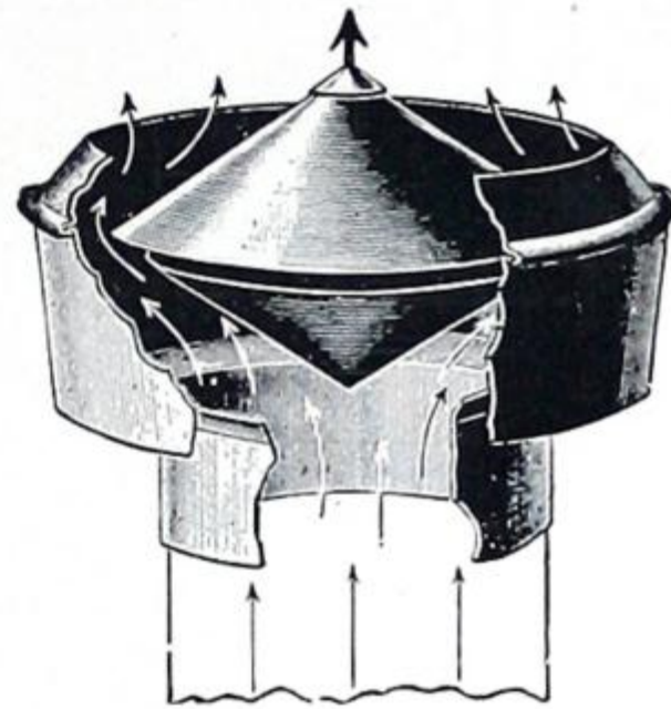
Fig. 228.—Broken View.
